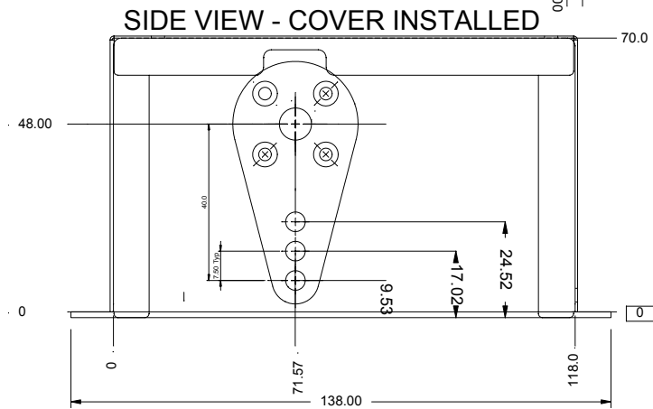
REV A BASEPLATE SHOWN
